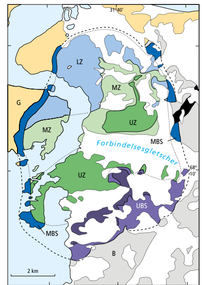
Simplified geological map of the Skaergaard intrusion.
